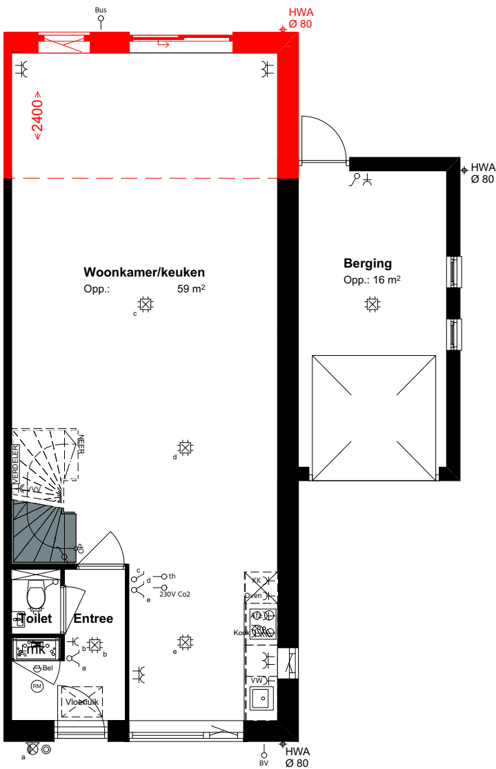
22 - 24 BEGANE GROND
