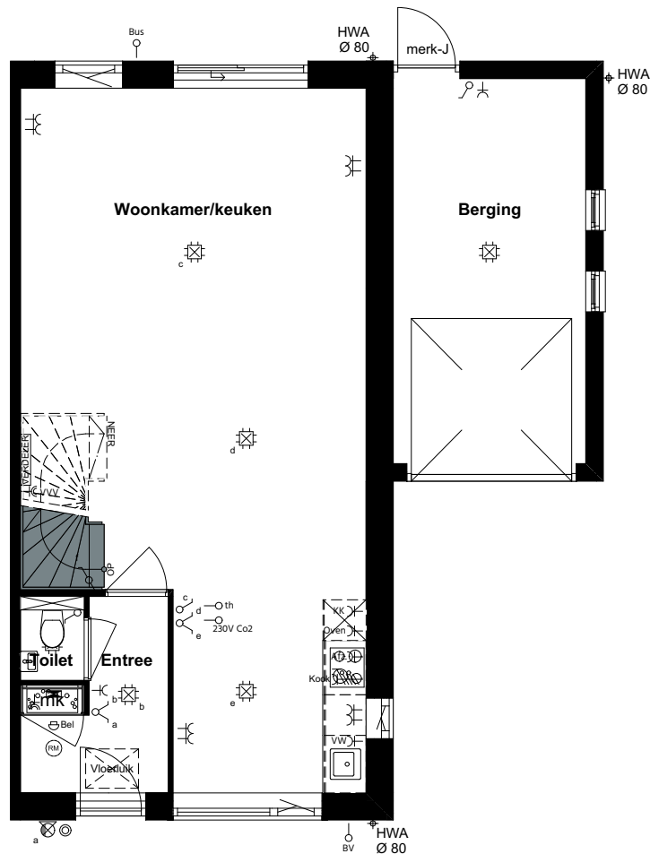
22 - 24 BEGANE GROND
