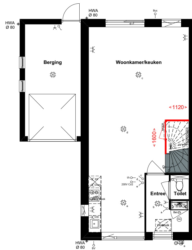
21 - 23 BEGANE GROND
