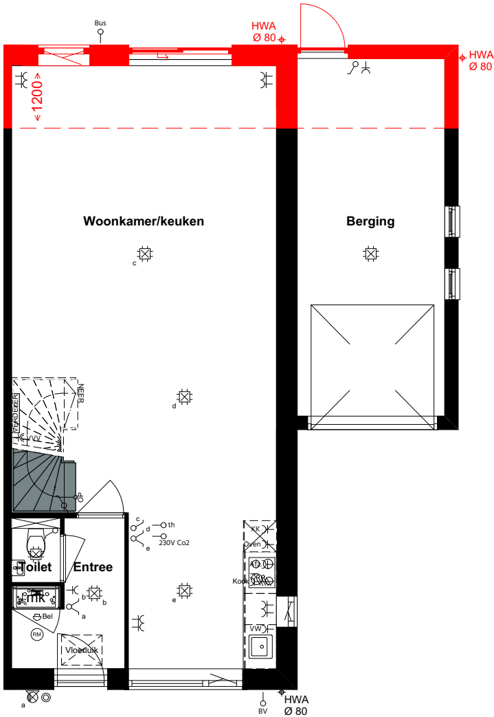
22 - 24 BEGANE GROND
