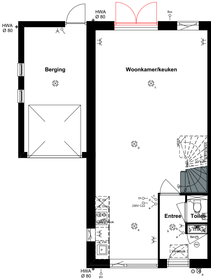
21 - 23 BEGANE GROND
