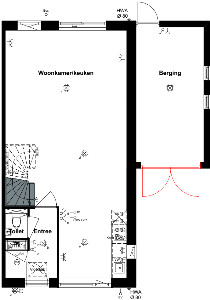
22 - 24 BEGANE GROND
