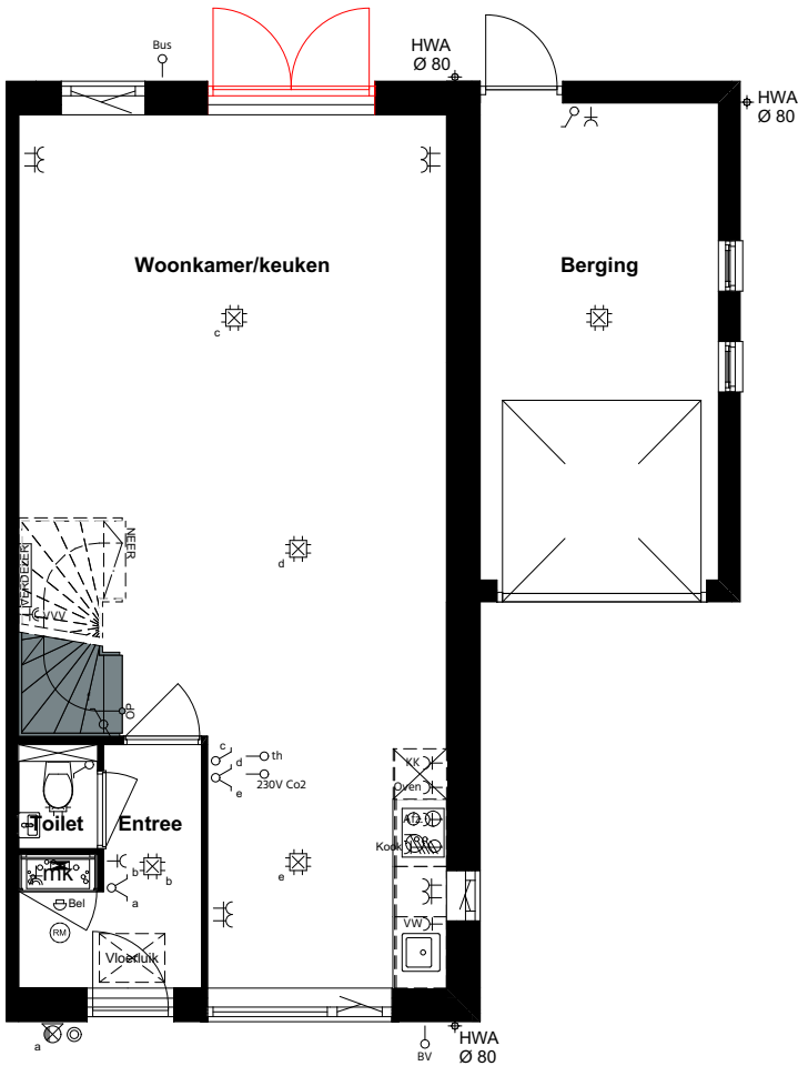
22 - 24 BEGANE GROND
