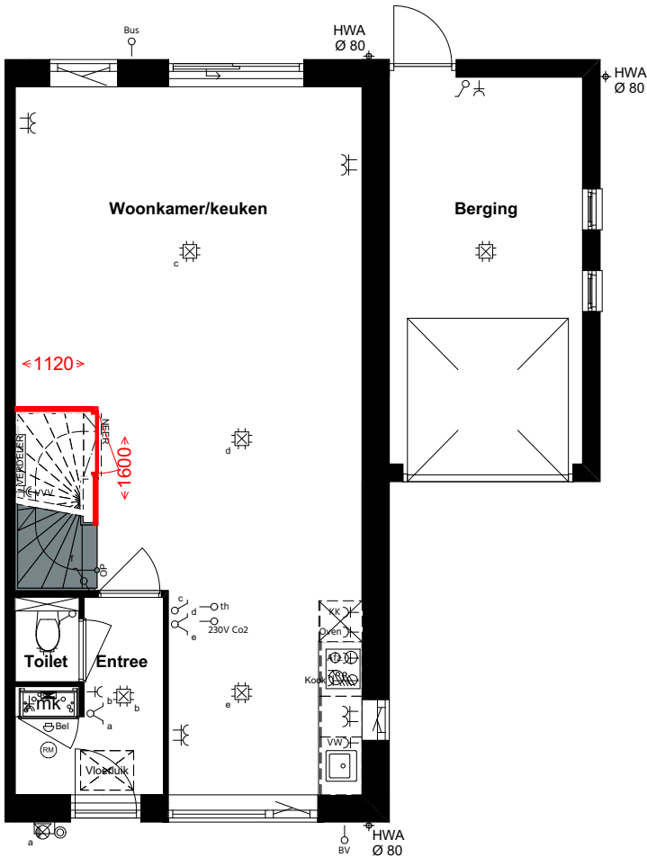
22 - 24 BEGANE GROND
