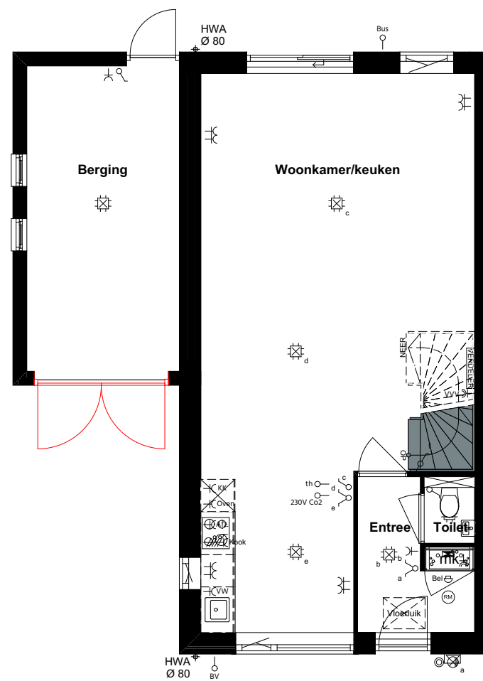
21 - 23 BEGANE GROND
