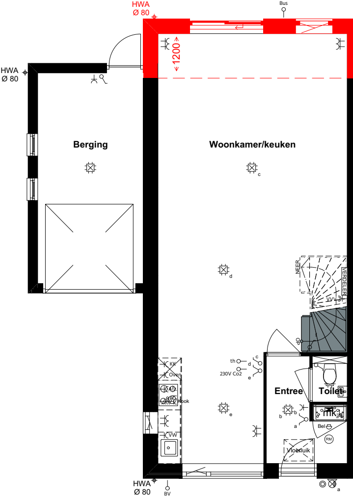
21 - 23 BEGANE GROND
