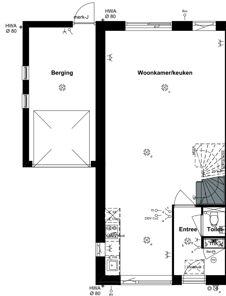
21 - 23 BEGANE GROND
