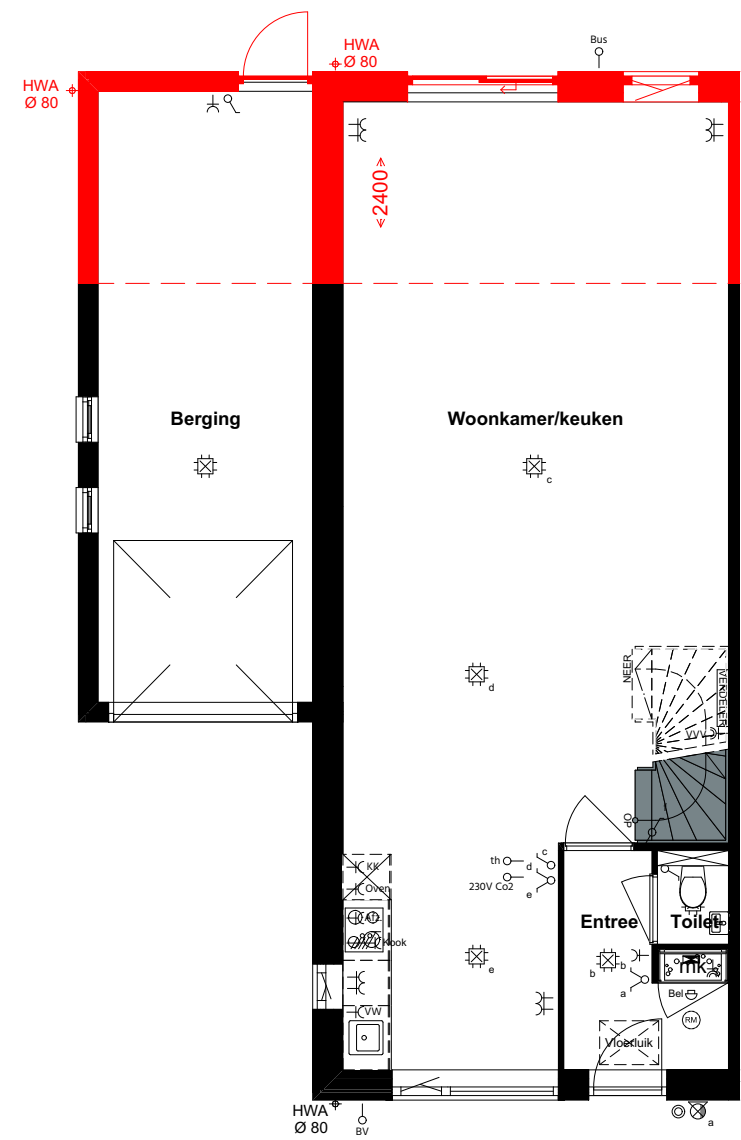
21 - 23 BEGANE GROND
