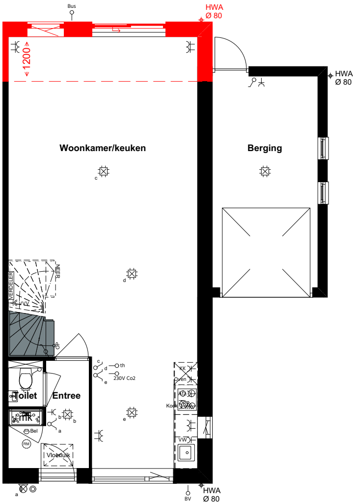
22 - 24 BEGANE GROND
