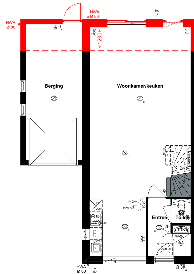
21 - 23 BEGANE GROND
