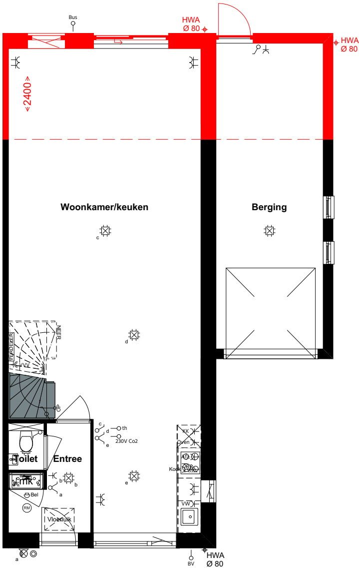
22 - 24 BEGANE GROND
